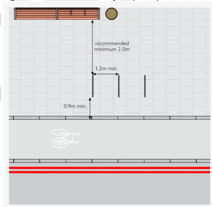
Figure 15 - Sheffield stand layout (LCDS)
